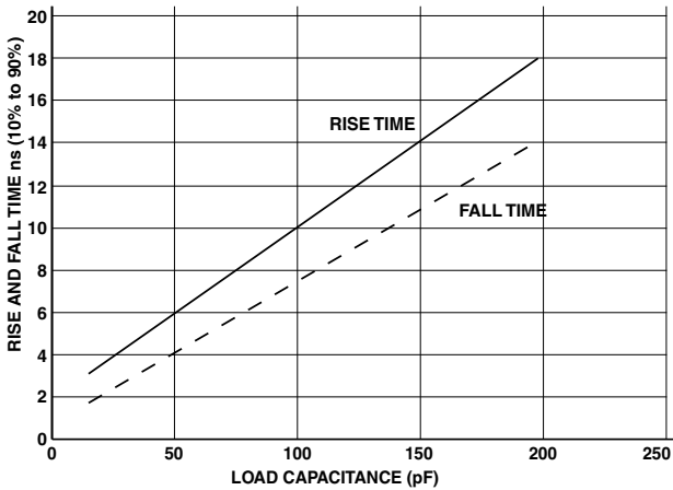
Figure 54. Typical Output Delay or Hold for Driver C at V_{DDEXT} Max
