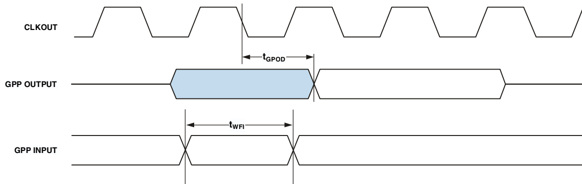
Figure 24. General-Purpose Port Timing
