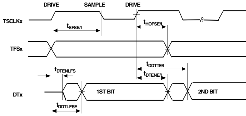
Figure 20. External Late Frame Sync
