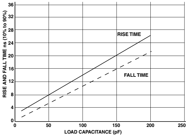
Figure 58. Typical Output Delay or Hold for Driver E at V_{DDEXT} Max
