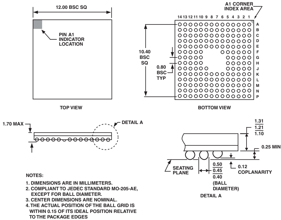
Figure 65. 182-Ball CSP_BGA (BC-182)
